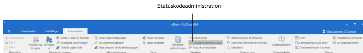
Figur 1: Statuskodeadministration
